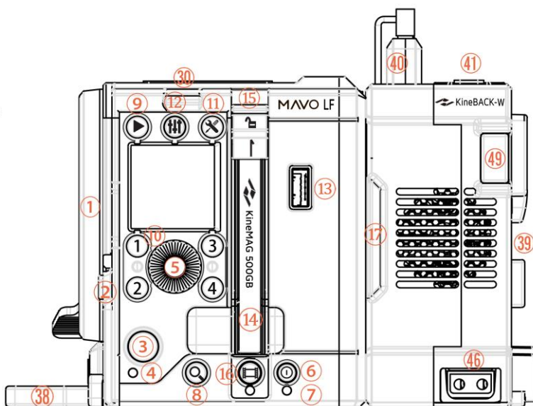
Left View of Body with KineBACK-W (KineMOUNT)
