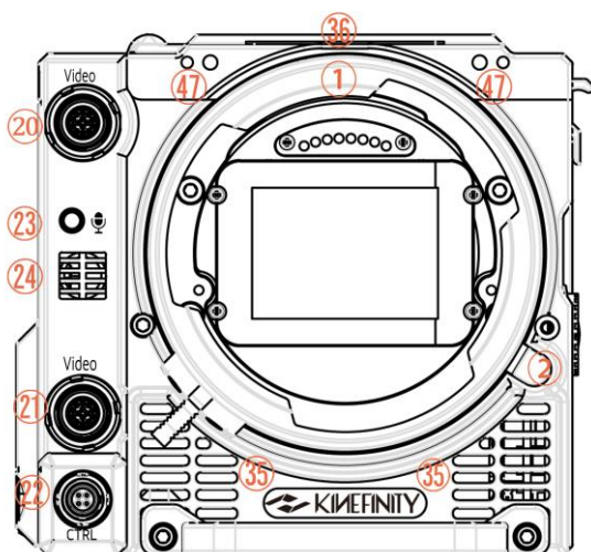
Front View (KineMOUNT)
